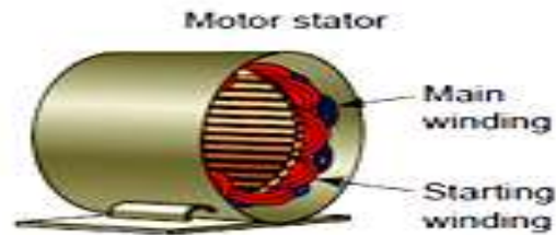
Motor stator
