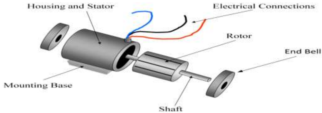
Split-phase motor
